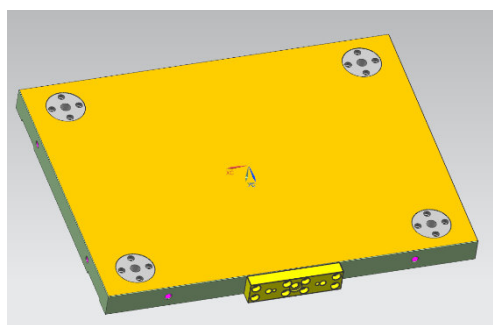
Fig. 3. Bottom side of the custom pallet
