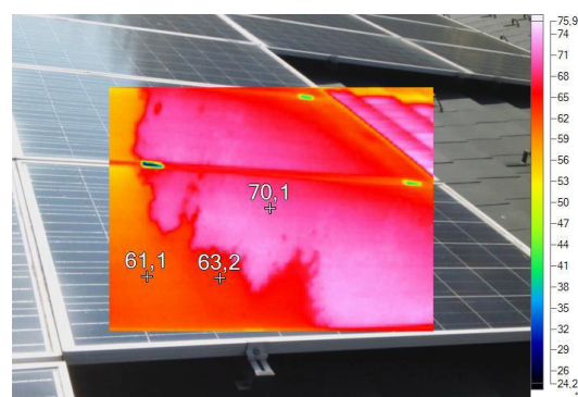
Figure 9: Incorrect measurement due to environmental reflection
