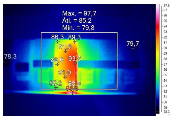
Fig. 7. Loaded circuit breaker
