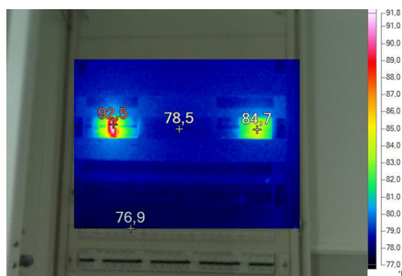
Fig. 6. Loaded circuit breaker board
