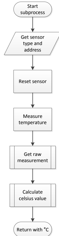
Figure 12: Matlab S-function flowchart
