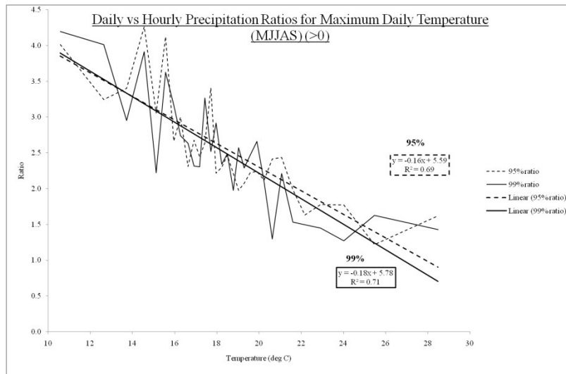
Figure 19. Daily/maximum hourly precipitation ratio in relation to maximum daily temperature for summer months (May-September). The bold-dashed line is the regression value of 0.69. The solid line is the regression value of 0.71
