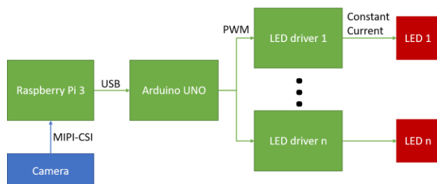
Figure 9. Block diagram of the hardware
