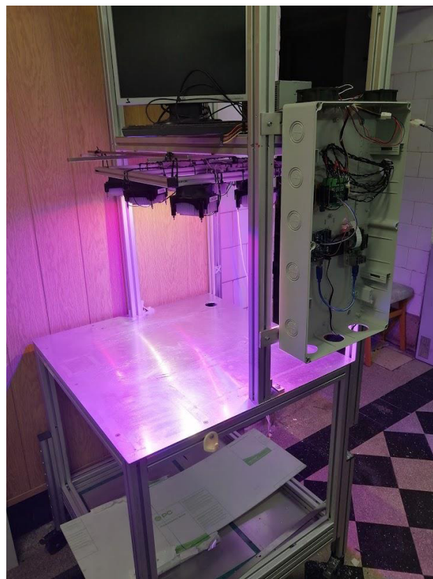
Figure 8. Picture of the test setup
