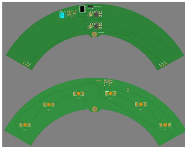
Figure 4. Front side of circular PCBs
