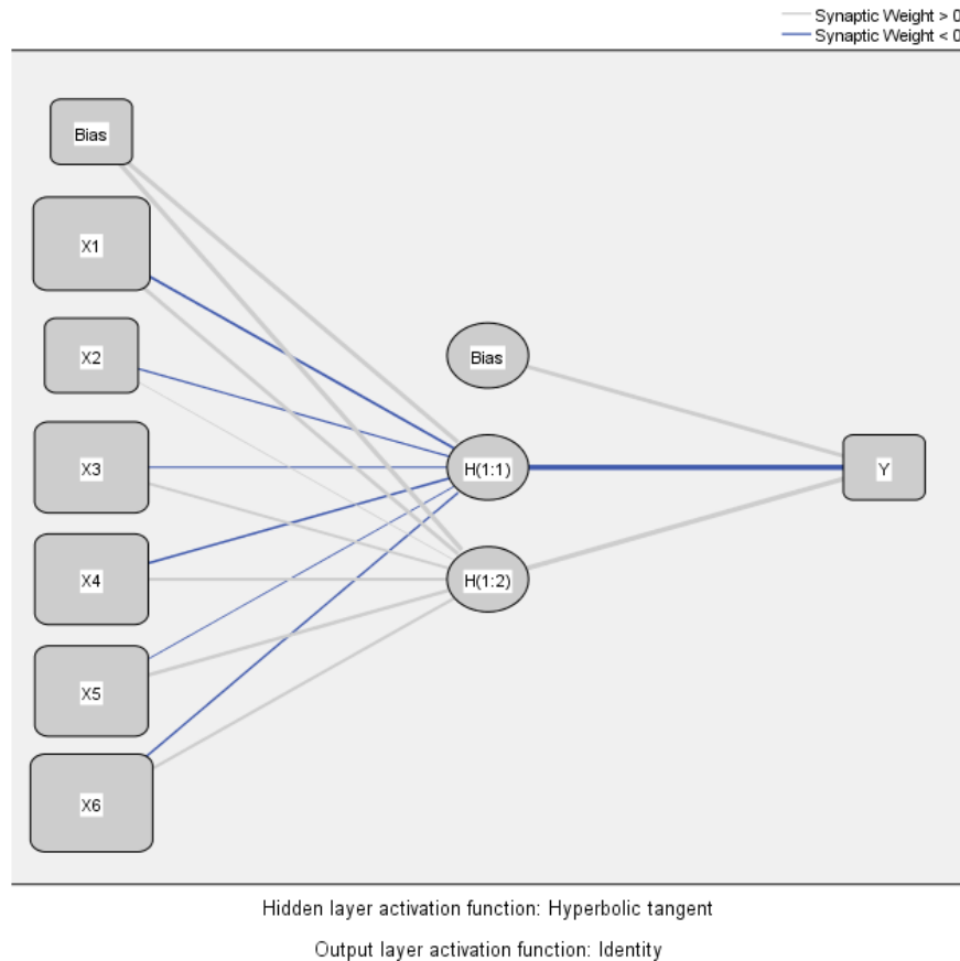
Figure 8 Artificial Neural Network.
