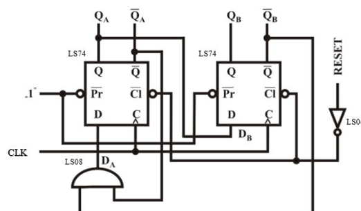
Figure 4 Sequential circuit with flip flop
