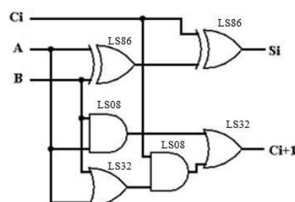
Figure 3 Full adder
