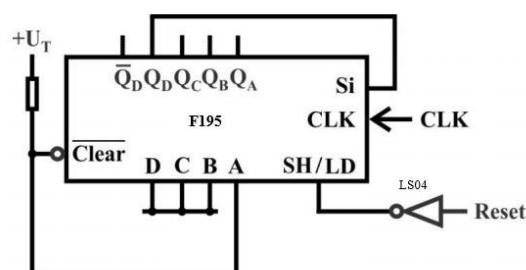
Figure 5 Ring counter
