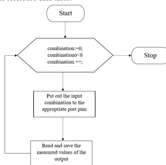
Fig. 17. The algorithm for the test of the combinational network
