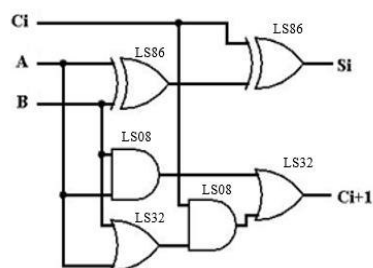
Fig. 7. Full adder
