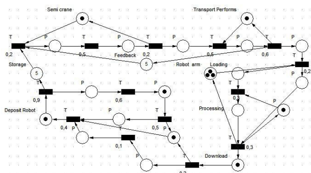
Figure 2. Classical structure modelled with Petri nets[7]
