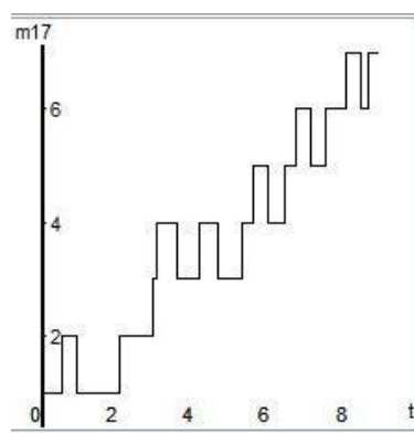
Figure 4. Transport blank in the classical system [7]
