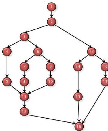
Figure 1 Execution graph
