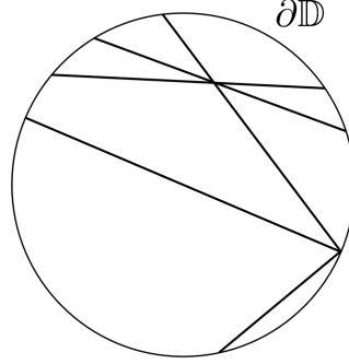
FIGURE 3.1: The pictorial representation of the Funk model (\mathbb{D}, F_F) : the geodesics are straight lines (chords) with ideal endpoints on the boundary \partial\mathbb{D} , see Shen [109, Example 9.2.1].
