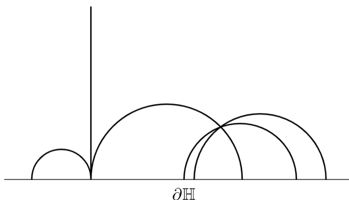
FIGURE 3.3: The pictorial representation of the Finsler-Poincaré upper half plane (\mathbb{H}, F_H) : the geodesics are straight Euclidean lines perpendicular to the x-axis and circular arcs intersecting the x-axis at Euclidean right angles (i.e., half-circles whose center is on the x-axis).
