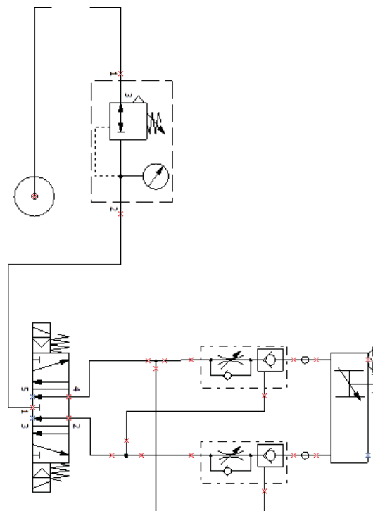
Figure 2: Pneumatic switching with 5/3 bistable valve
