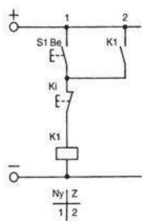
Figure 3: Self-holding circuit
