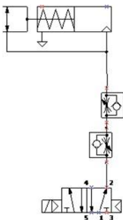
Figure 1: Control with 3/2-way valve, with placement of throttle check valves
