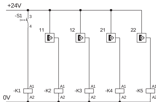
Figure 6: Sensor circuit
